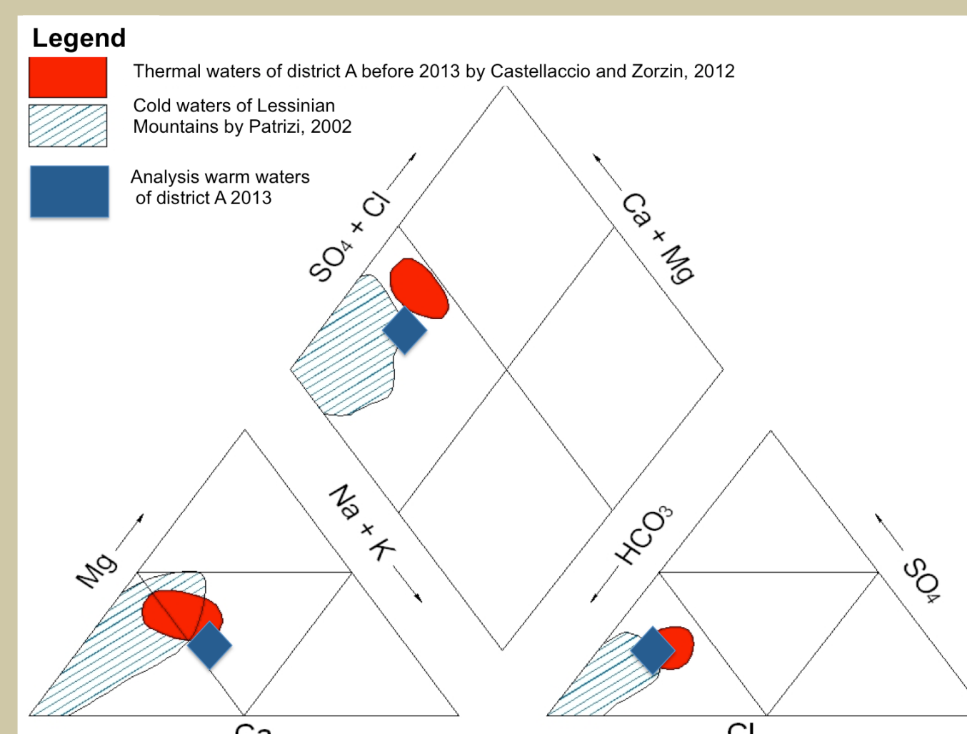
Fig.3a – Chemical analysis of wells and springs district A. In evidence the close correlation between analysis of Lessinian mountains cold waters and warm waters 2013 data
