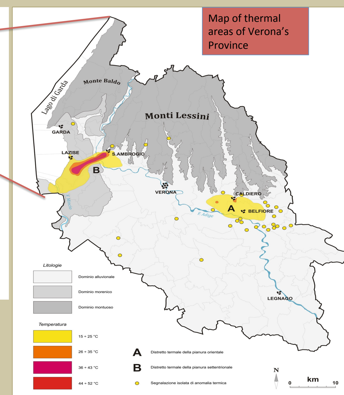
Fig.1b – Thermal district map of the Verona Province (Castellaccio and Zorzin 2012)
